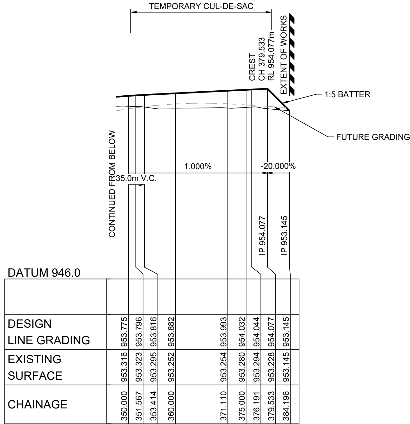
LONGITUDINAL SECTION ROAD A HORIZONTAL SCALE 1:500 VERTICAL SCALE 1:100
