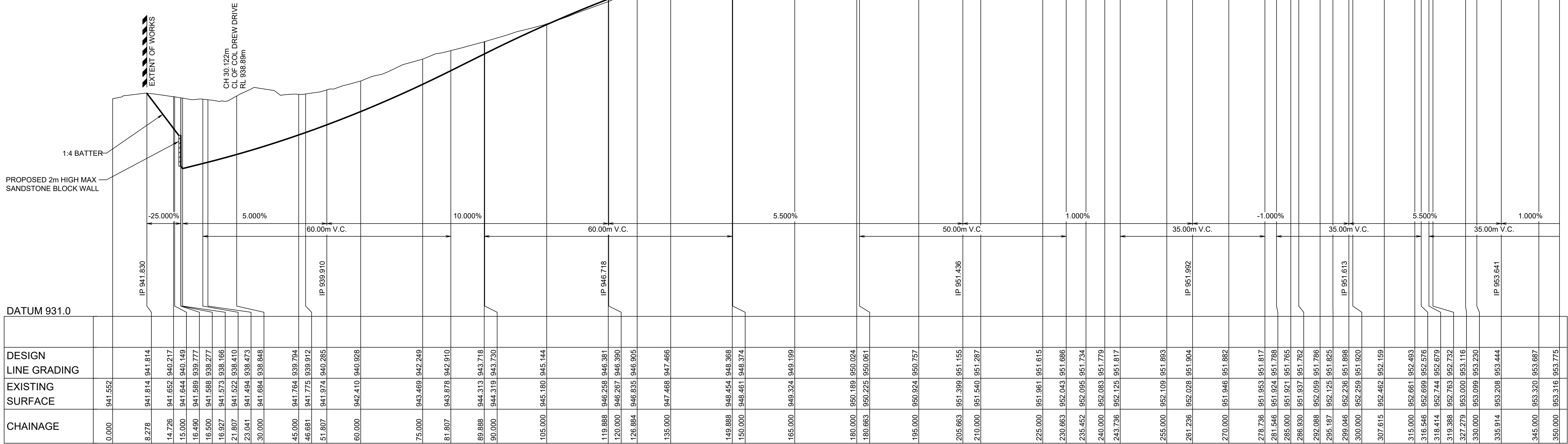
LONGITUDINAL SECTION ROAD A HORIZONTAL SCALE 1:500 VERTICAL SCALE 1:100
