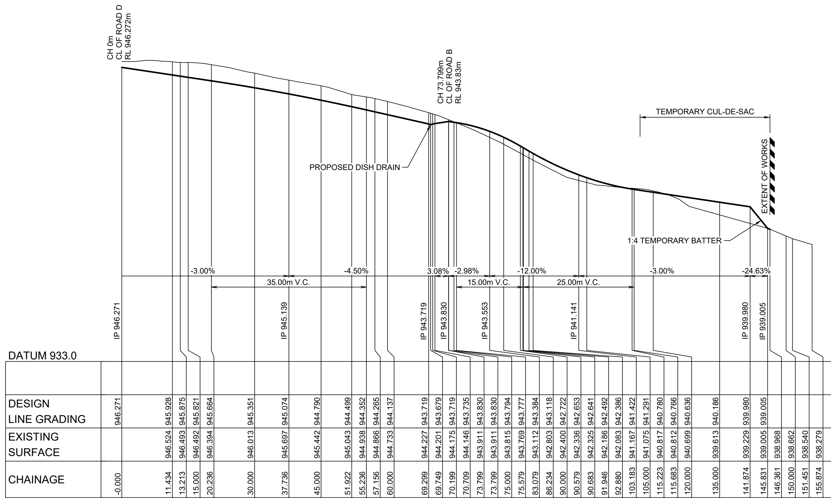
LONGITUDINAL SECTION ROAD C HORIZONTAL SCALE 1:500 VERTICAL SCALE 1:100
