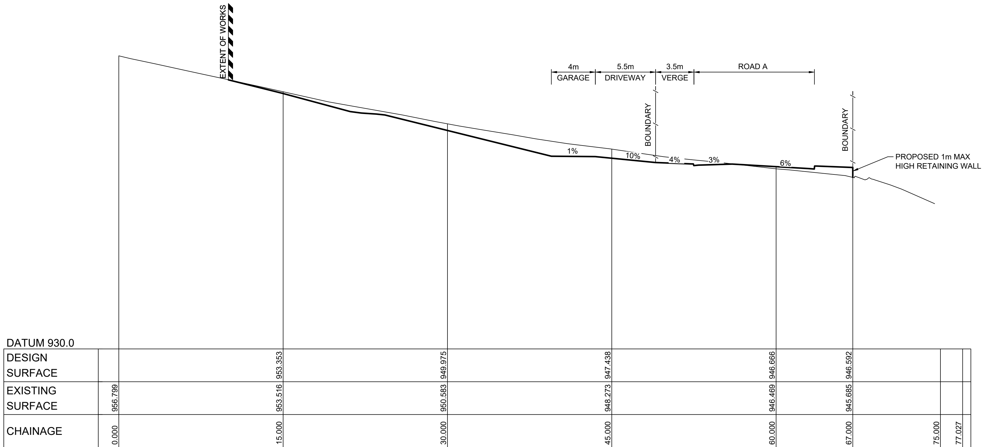
SECTION C SCALE H 1:200 V 1:200 CD010
