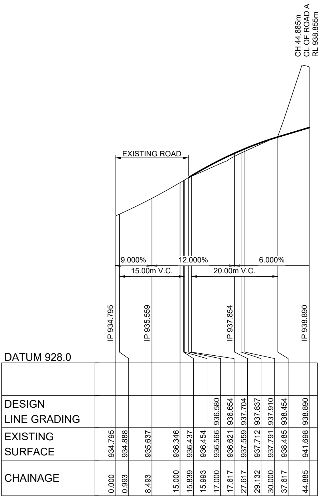
LONGITUDINAL SECTION COL DREW DRIVE HORIZONTAL SCALE 1:500 VERTICAL SCALE 1:100
