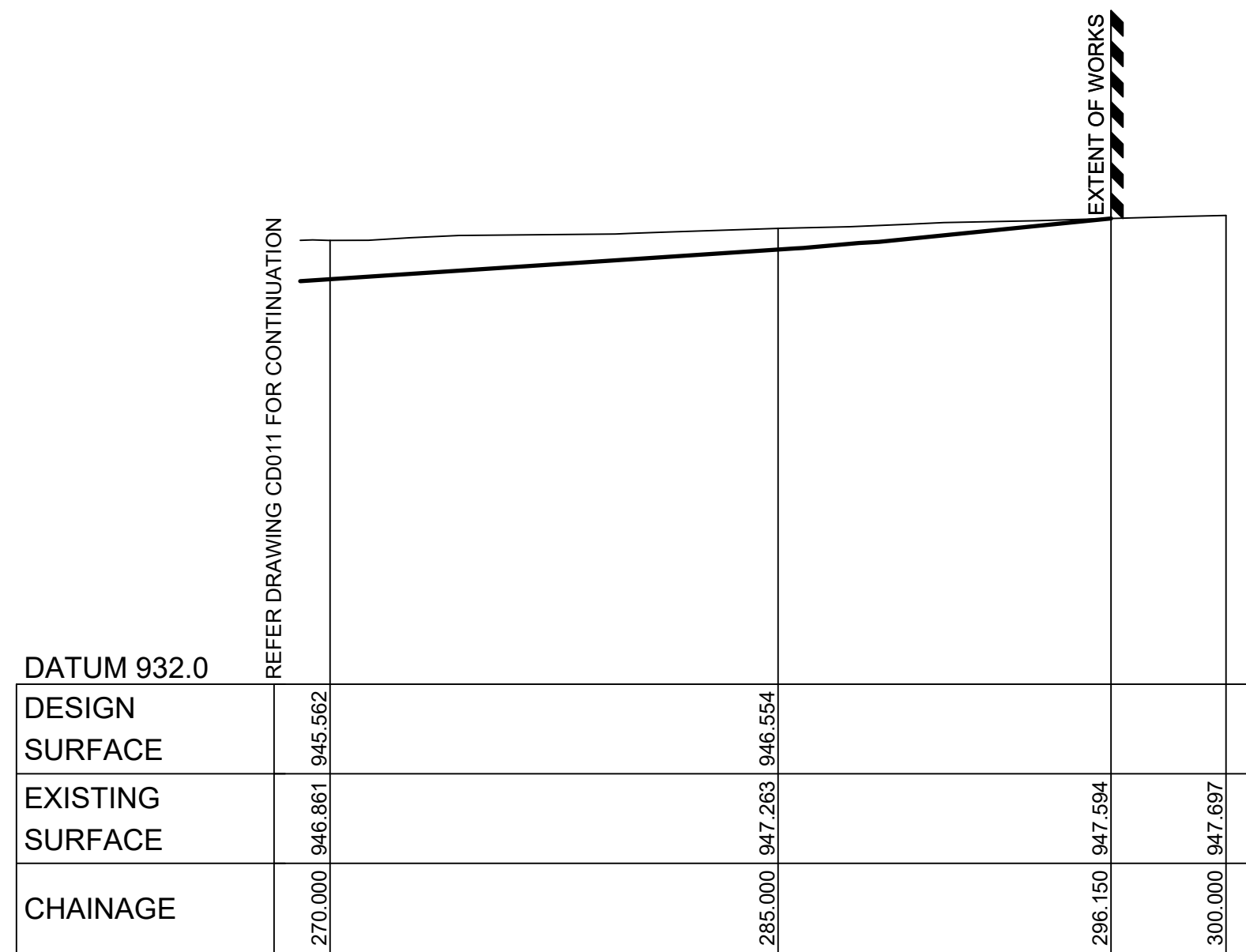
SECTION A SCALE H 1:200 V 1:200 CD010
